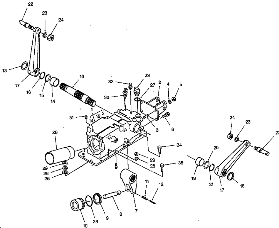
HYD-CYLNDER
