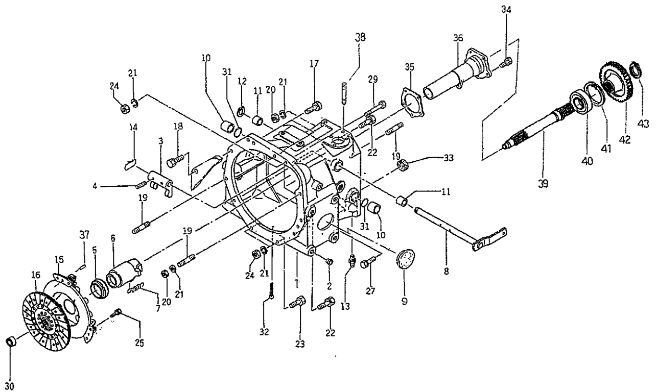
CLUTCH CASE ; MECHA
