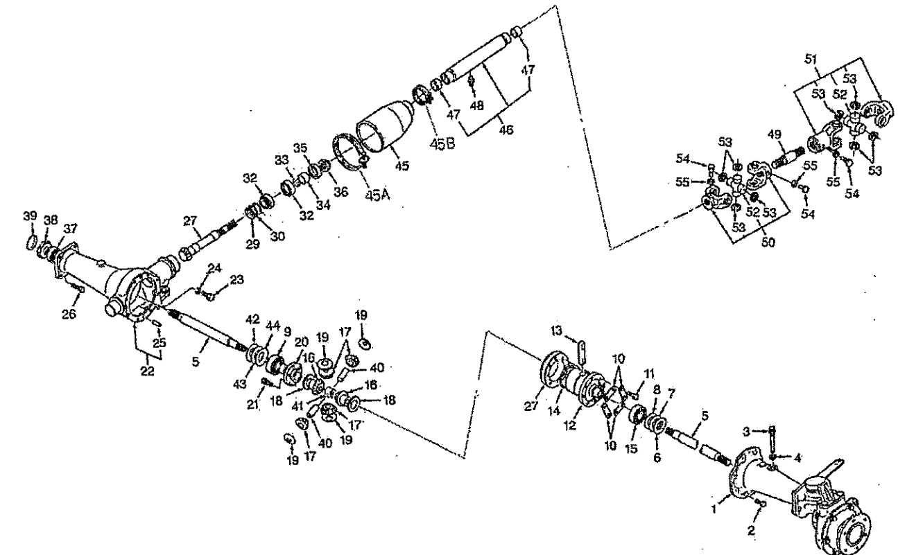
FIG.202 フロント デフ FRONT DIFF
