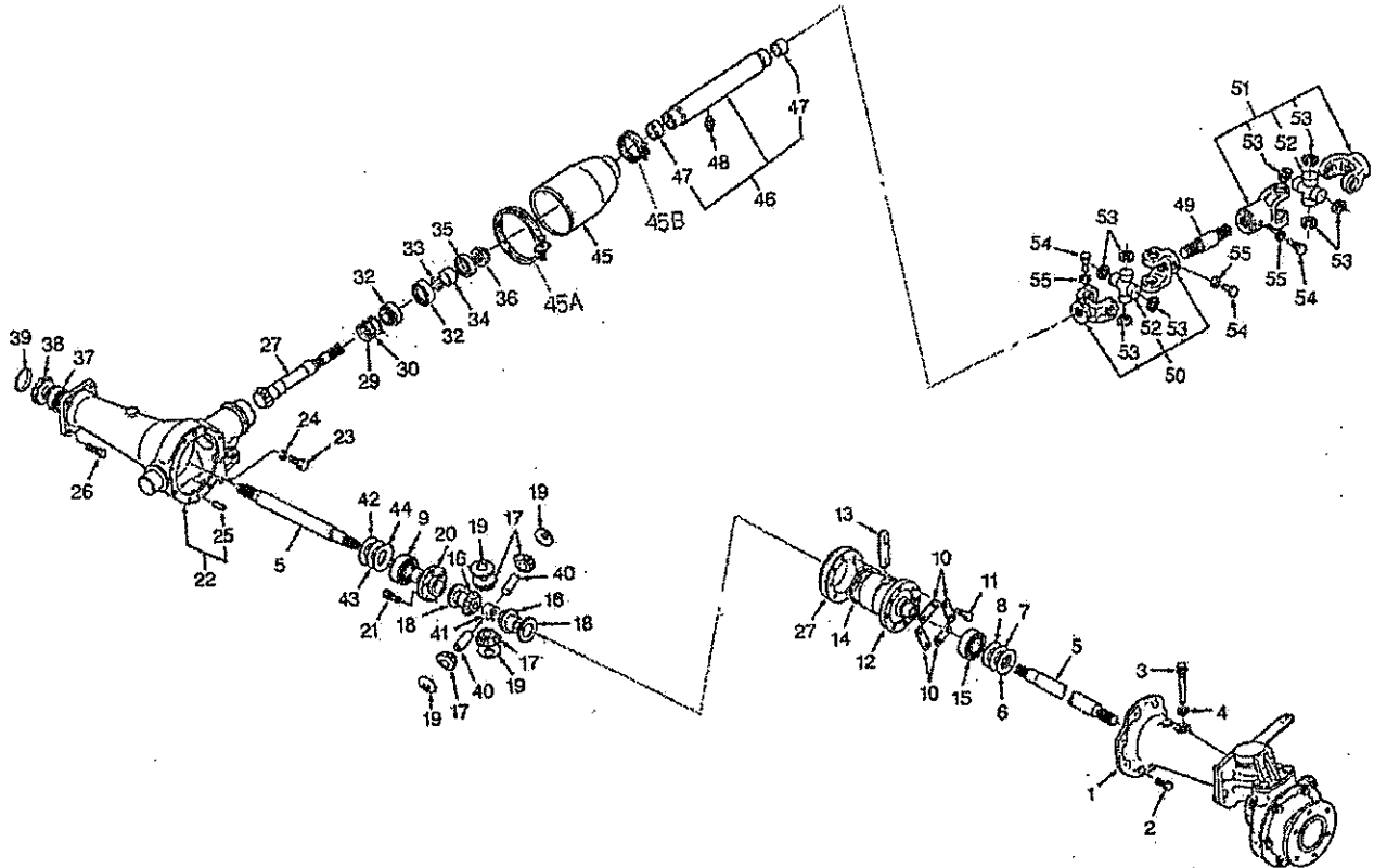
FIG.202 フロント デフ FRONT DIFF
