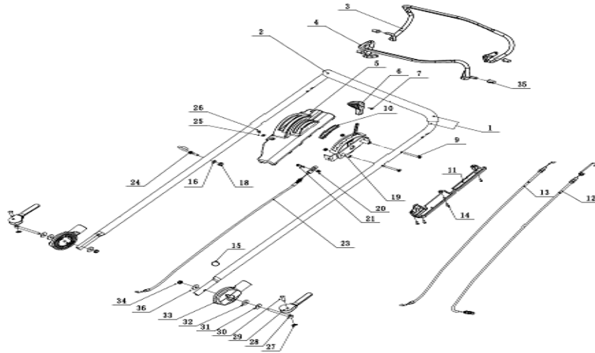
FIG.6 Handle And Controls
