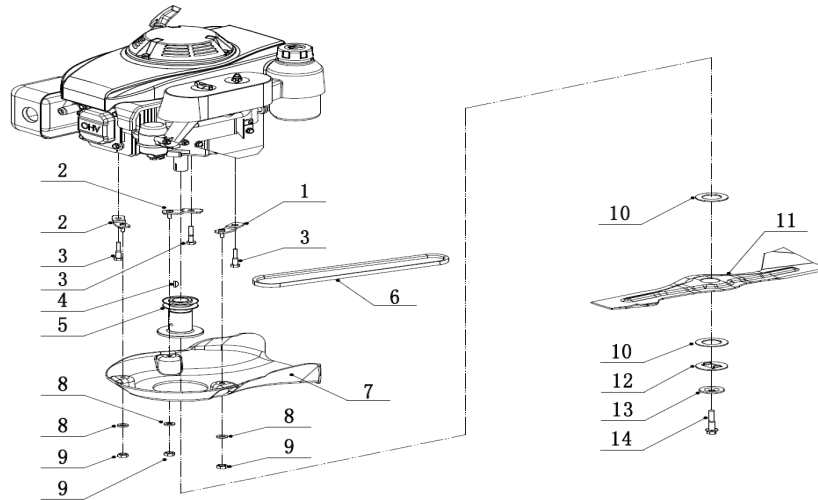
FIG.3 Blade System
