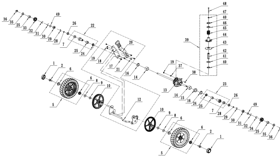
FIG.5 Rear Axle
