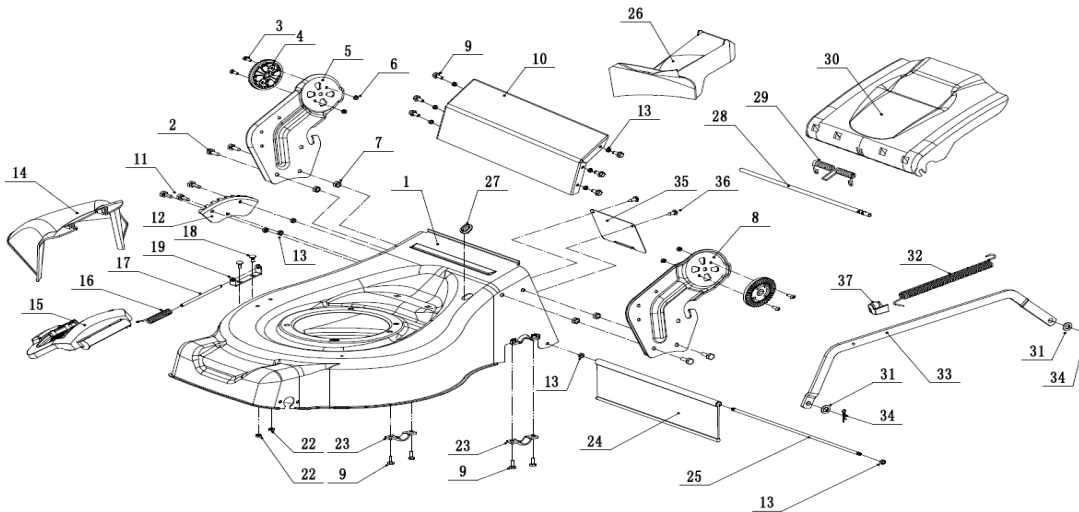
FIG.2 Main Body
