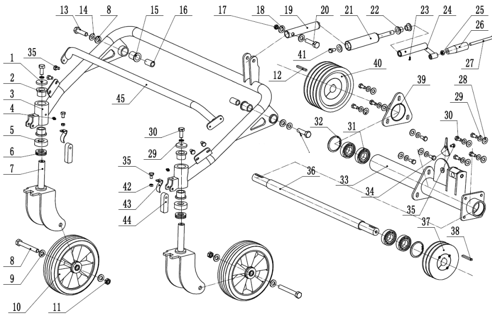
FIG.4 Front wheel bracket
