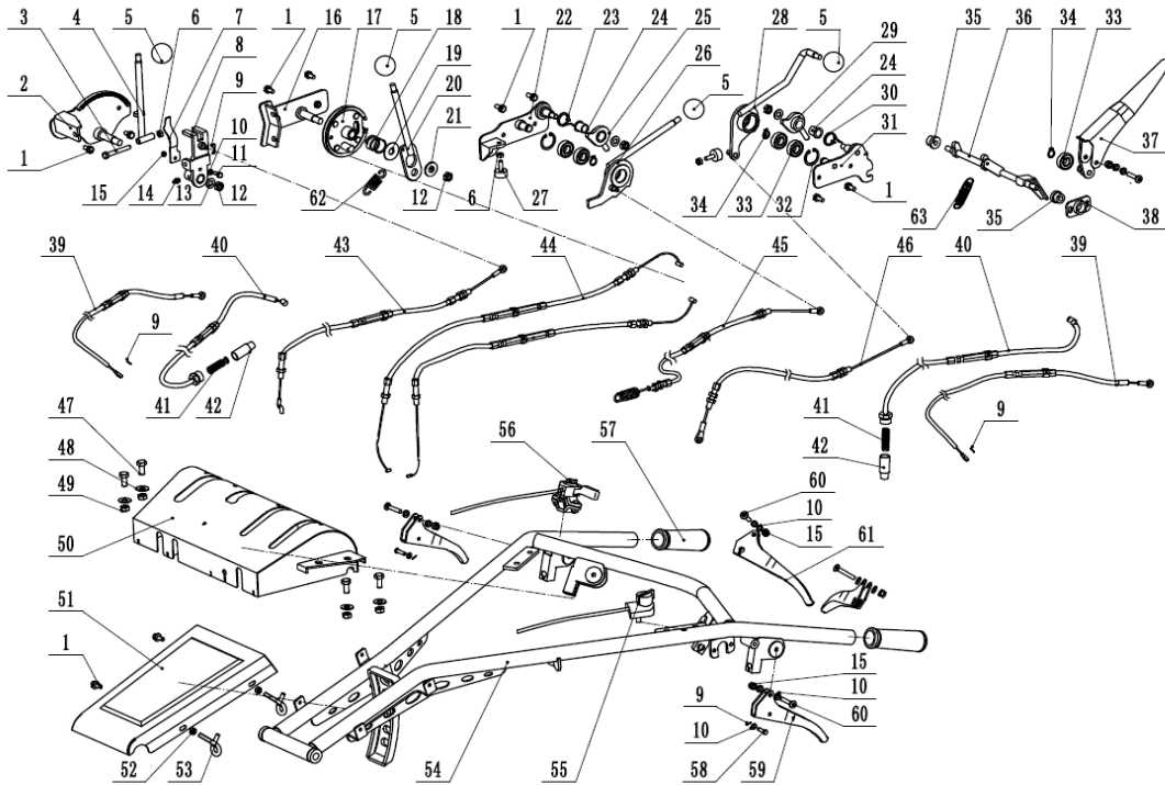
FIG.1 Handle and controls
