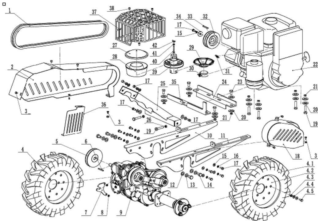
FIG.5 Engine part
