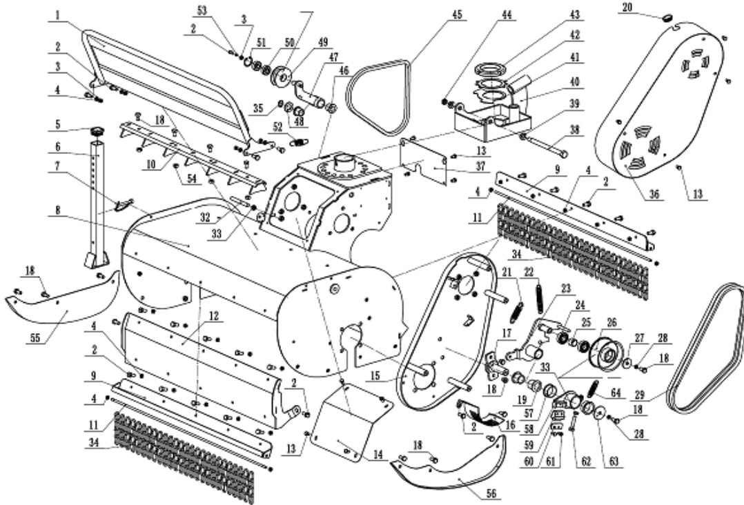
FIG.2 Main Body
