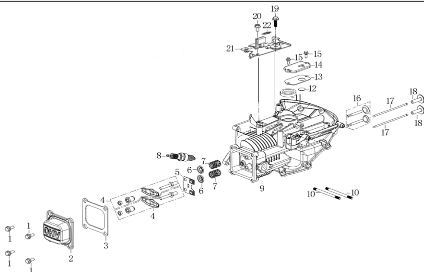
FIG. 1 CRANK CASE
