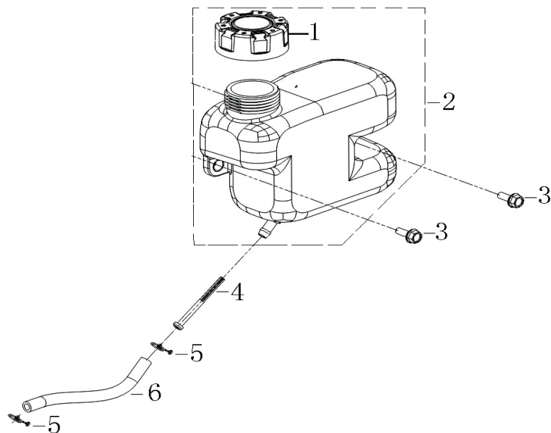
FIG. 8 FUEL TANK
