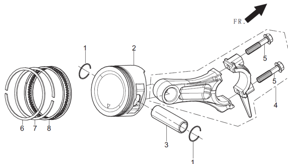
FIG.5 RING SET,OIL / ROD,CRANKSHAFT CONNETING 油环组合/曲柄连杆组件 ( E03 )
