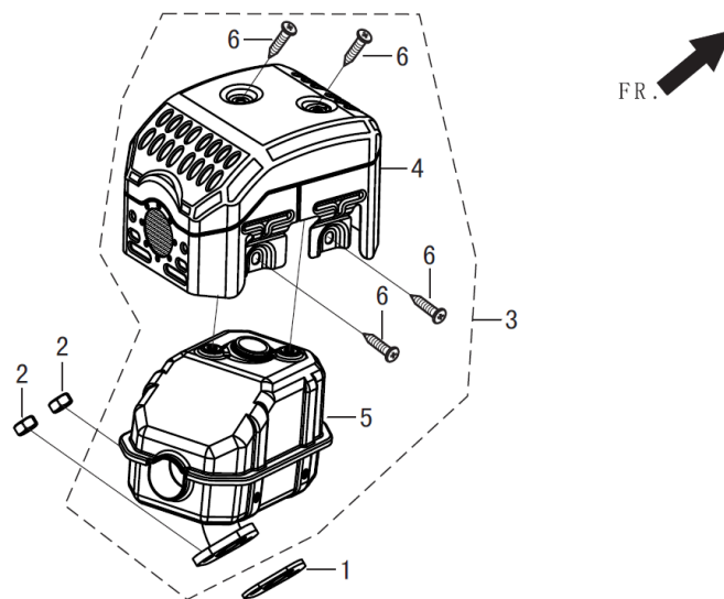
FIG.11 MUFFLER ASSY. 消声器部件 ( F04 )
