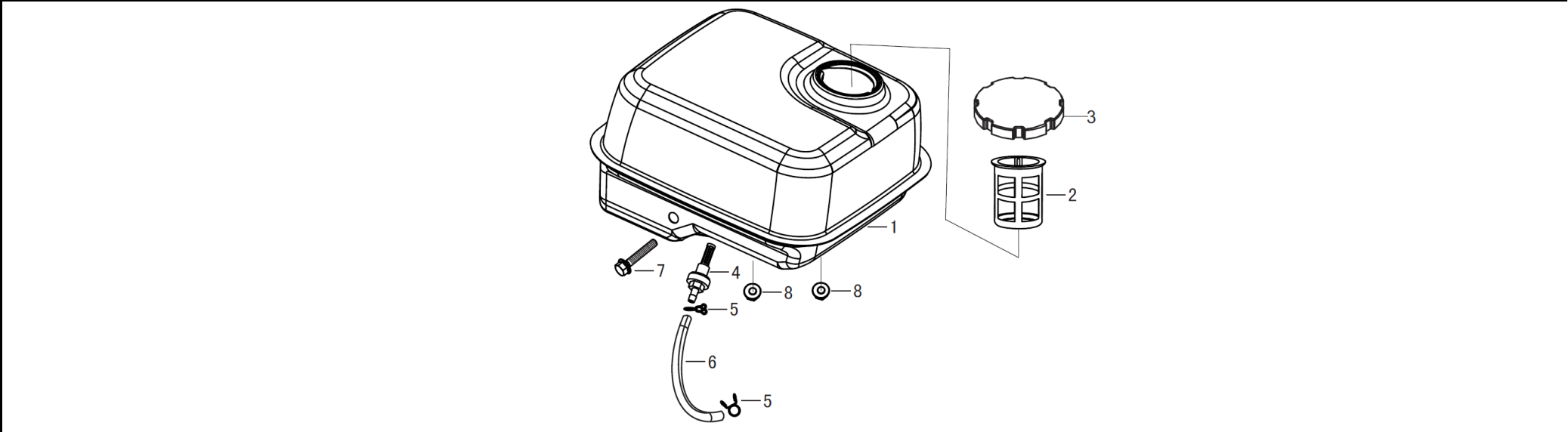
FIG.12 TANK ASSY, FUEL 油箱部件 ( F01 )
