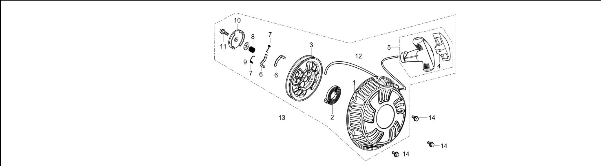
FIG.7 STARTER,RECOIL 手起动组件 ( E08 )
