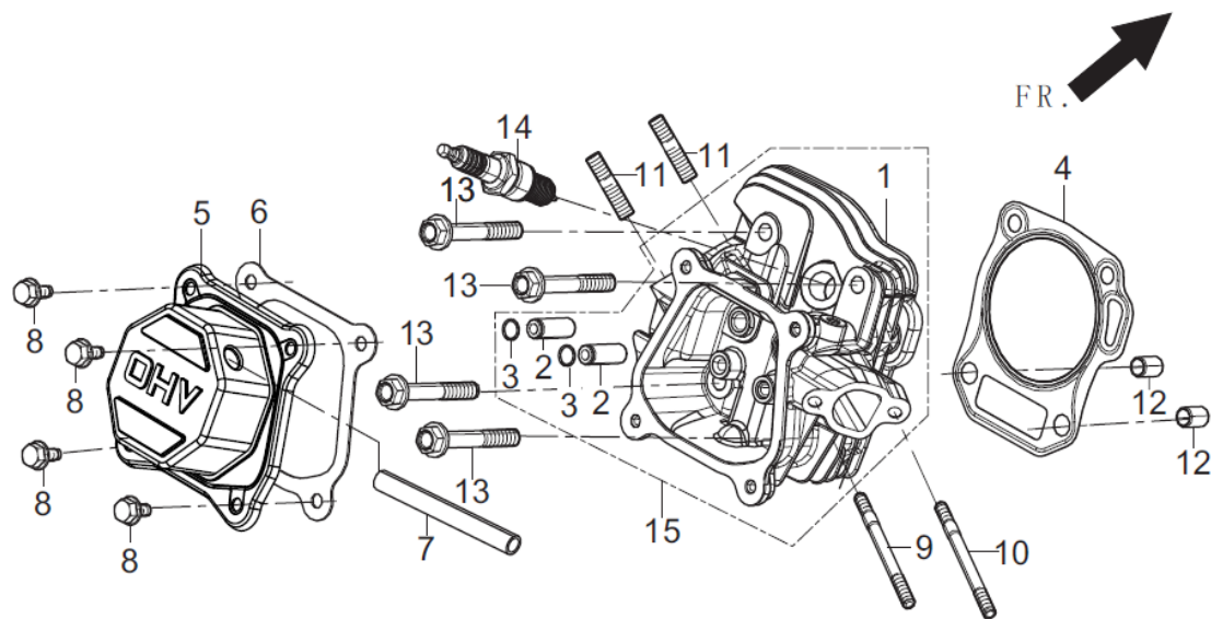
FIG.1 HEAD SUBASSEMBLY, CYLINDER / PLUG,SPARK 气缸头部件/火花塞 (E04)
