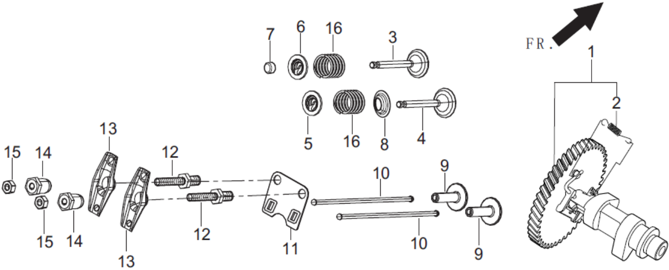
FIG.6 TRAIN,VALVE / CAMSHAFT SUBASSEMBLY 配气机构组件/凸轮轴 ( E05 )
