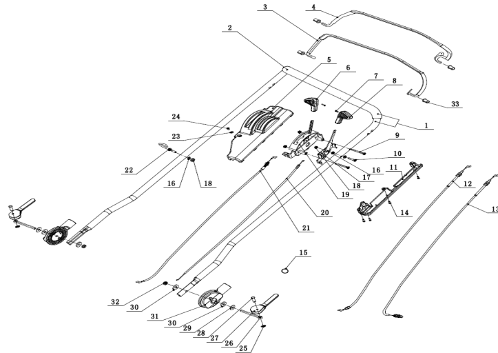
FIG.6 Handle And Controls
