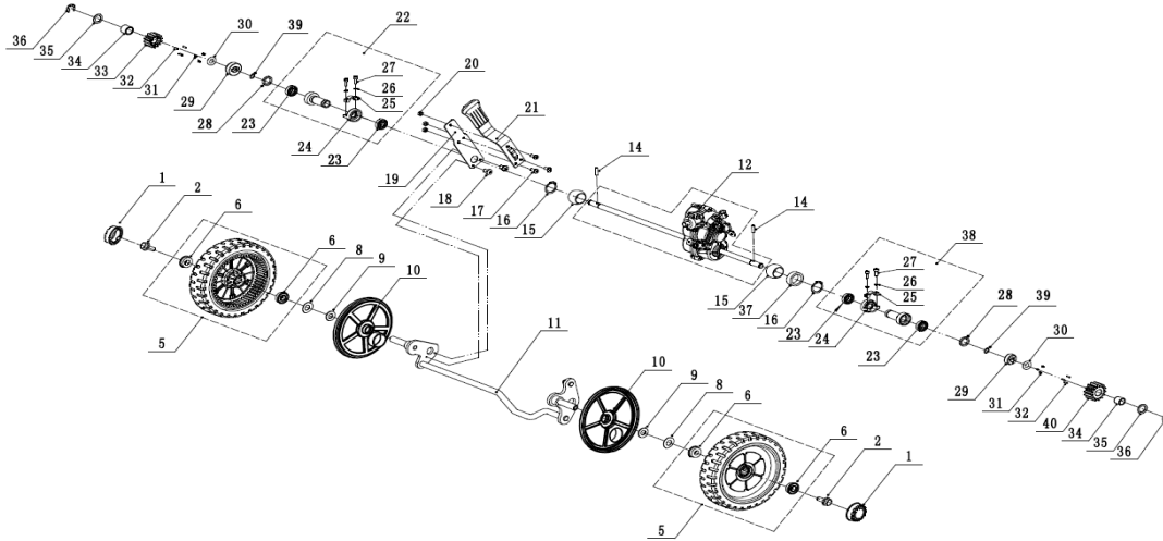
FIG.5 Rear Axle
