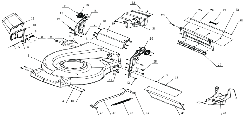
FIG.2 Main Body
