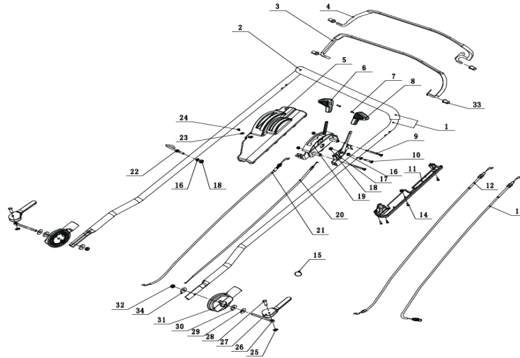
FIG.6 Handle And Controls
