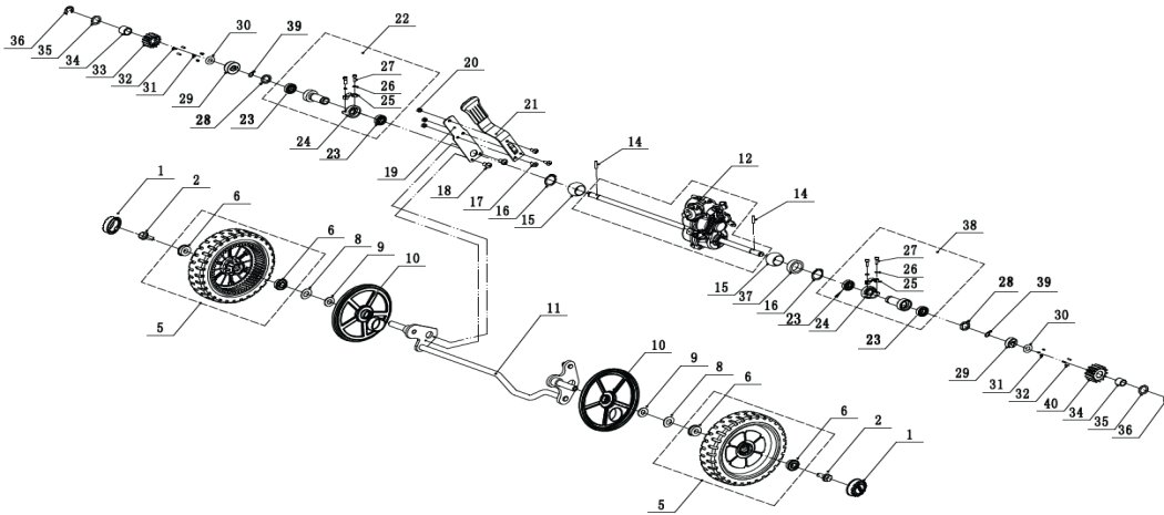
FIG.5 Rear Axle
