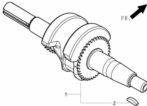
FIG.4 ROD,CRANKSHAFT CONNETING(E03)
